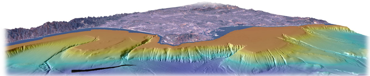
Caption: Overall perspective view of the Los Angeles Margin and Basin looking northeast. The distance across the bottom of the image is about 100 kilometers with a vertical exaggeration of 6 times. The margin is bisected by a series of large underwater canyons, channels, and gullies. Underwater landslides occur along the steep slope off the Palos Verdes Peninsula (far right) depositing large blocks into the deeper basin.
