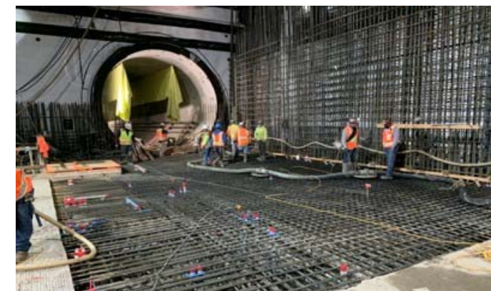
Concrete Placement at Wilshire/La Cienega Station (West)
