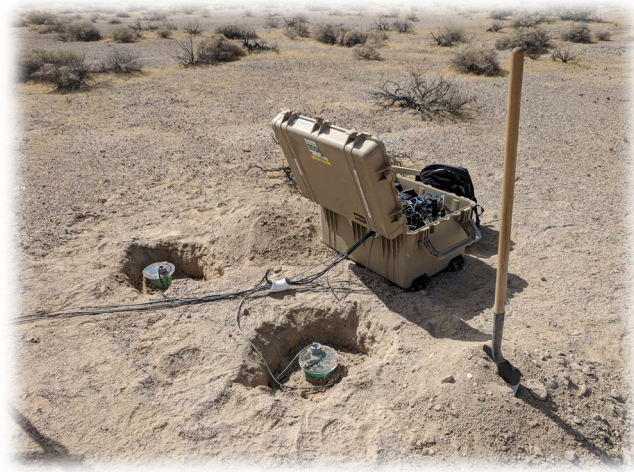
Caption: Two portable sensors: a strong motion sensor (to record strong shaking that can be felt) and a broadband sensor (to record weak motion for detecting small earthquakes) buried into the ground to detect earthquakes. These stations can be quickly deployed and send real-time data back to the USGS via cellular telemetry immediately after they are installed.
