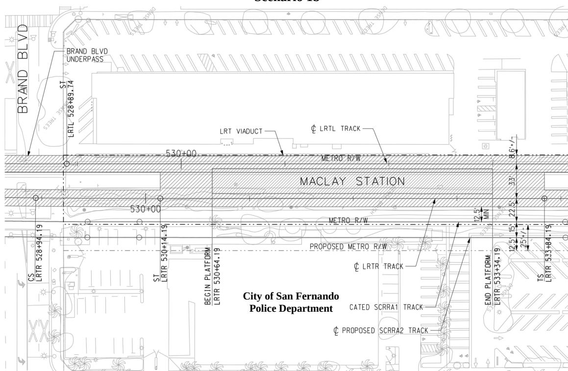
Figure 5-2: Permanent Right-of-Way (ROW) Impact at the City of San Fernando Police Department, Scenario 1b
